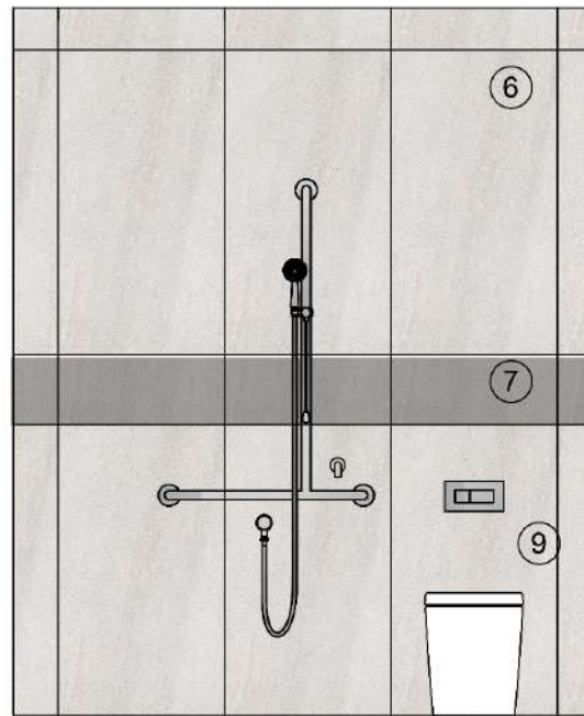
ELEVATION - SHOWER + WC
